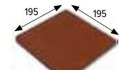
Esquina/REX 20 Stair-tread corner 20 195x195x13 mm
