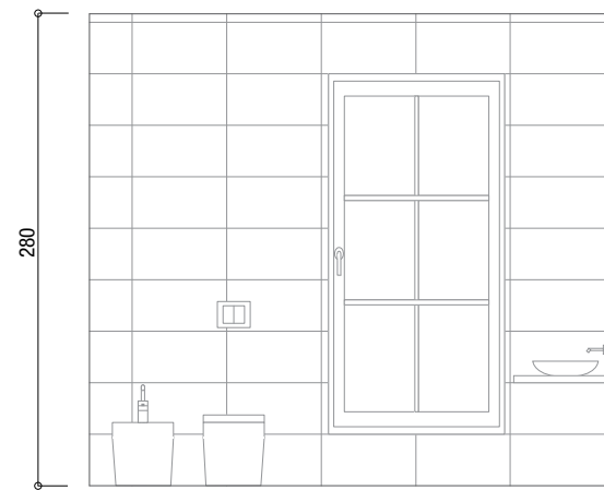
Wall A
